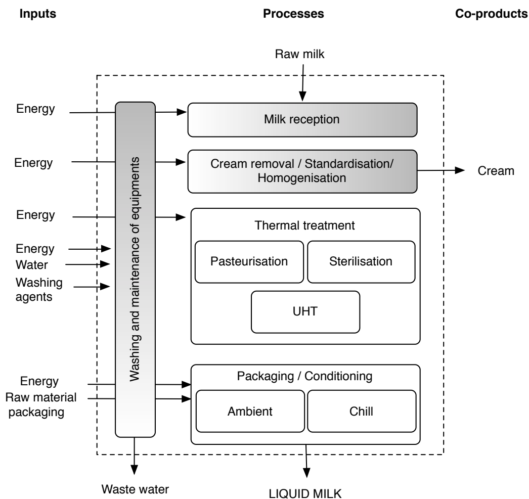
Figure 5: Process diagram for liquid milk
